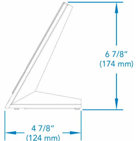
MXT-1000 (Right View)
