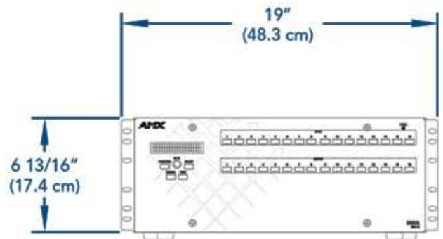
AVS-ENOVADGX16-ENC (Front View)
